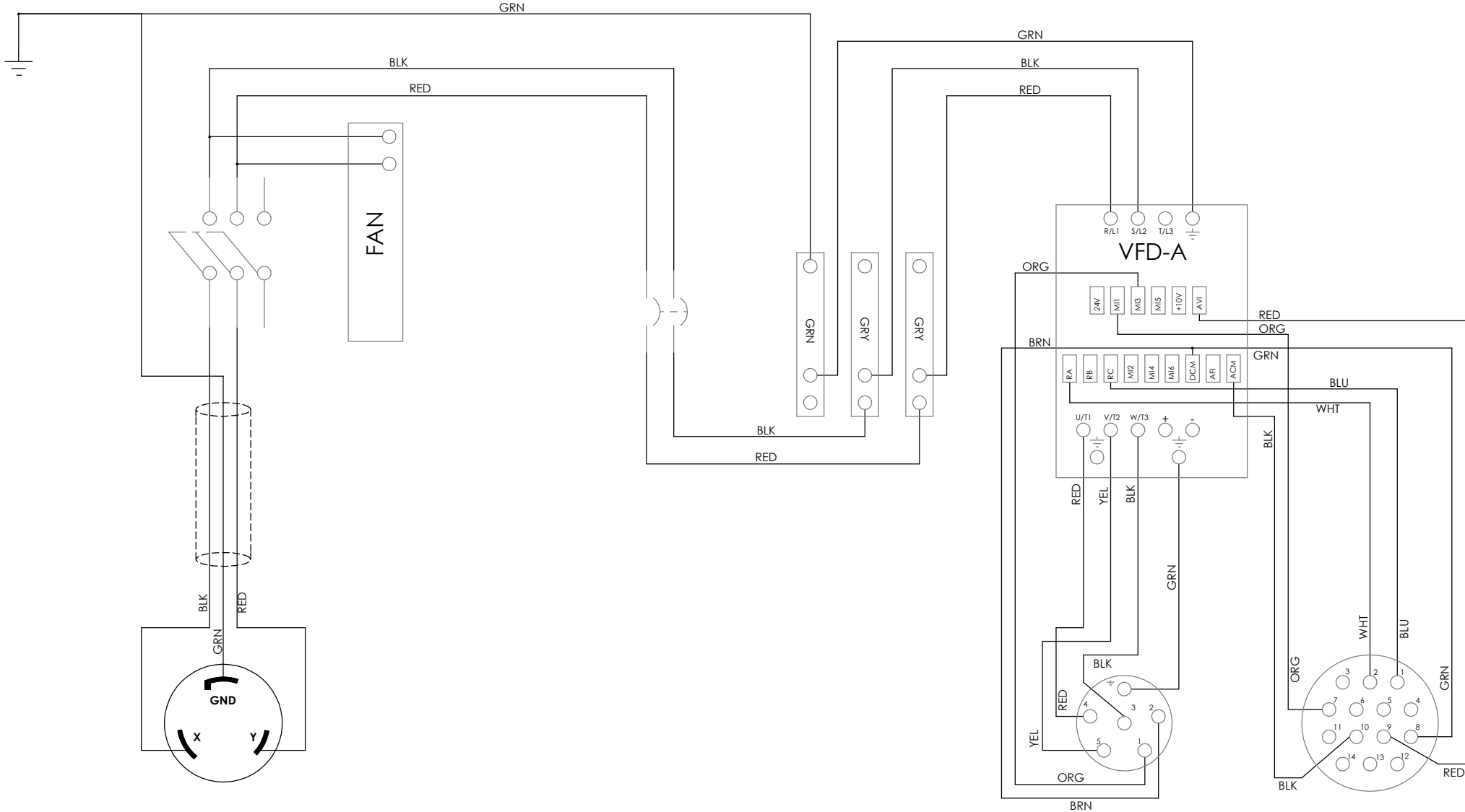
L6-30P 200-240 VAC
